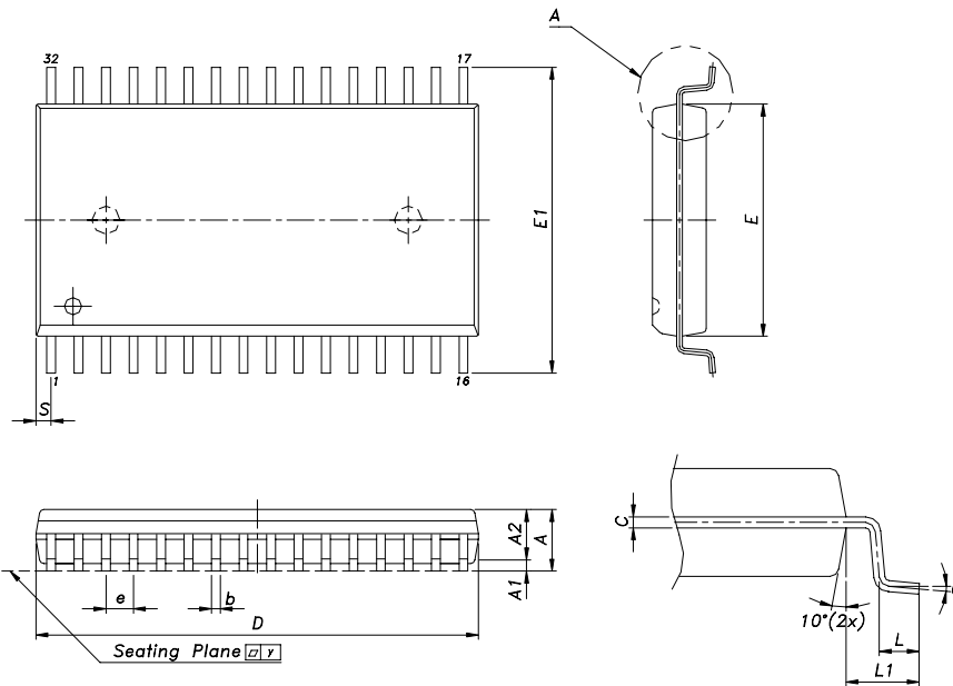
DETAIL: A(SCALE 2/1)
