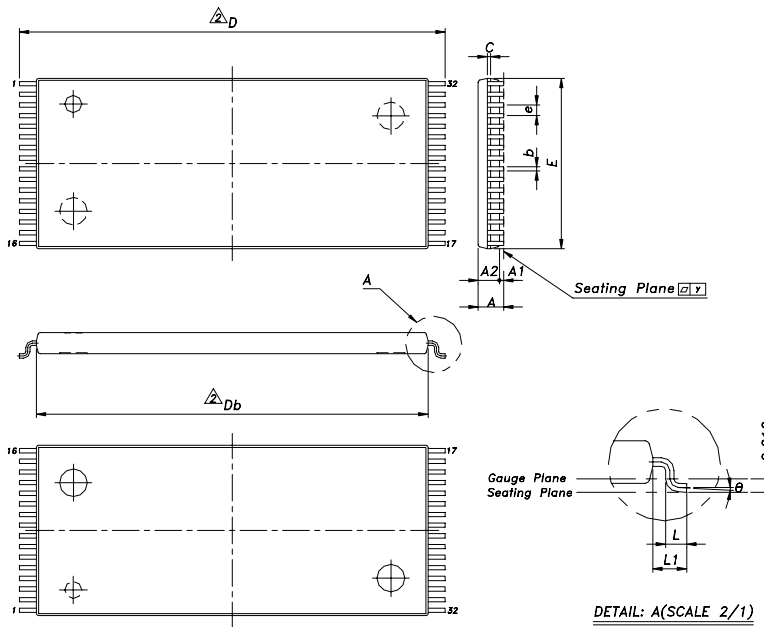
TSOP-32
